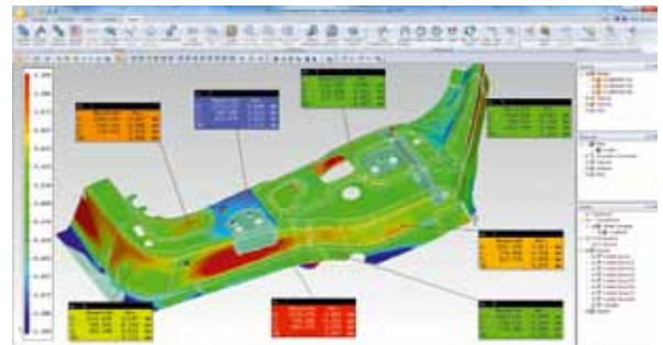
Laser scanning enables full part-to-CAD inspection
