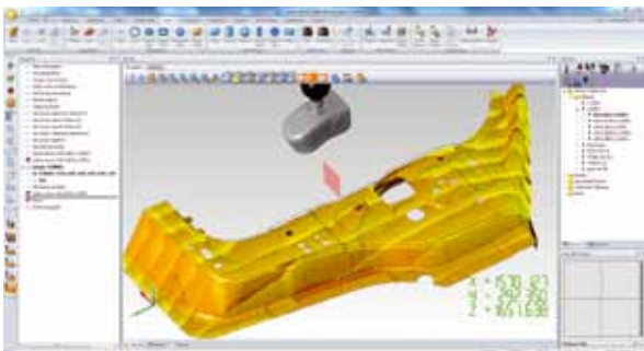
Measured point clouds are immediately visualized. Geometric features can be automatically extracted from a surface point cloud scan.
